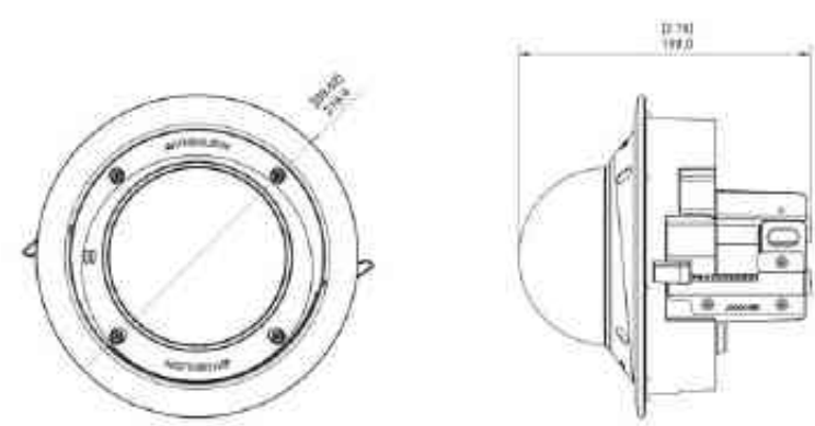
H6A Dome Camera with In-Ceiling Mount (CLADP-1001)
